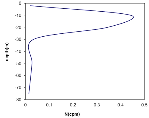
Figure 3. Calculation of buoyancy frequency using the data sets of a device installed in the Persian Gulf near Hormuz Strait at 2001.
