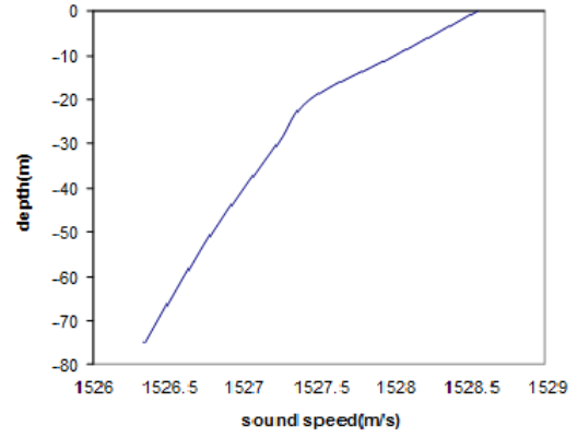
Figure 2. Calculation of sound speed profile using the data sets of a device installed near Hormuz Strait at 2001.
