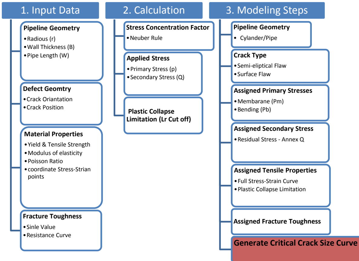
Figure 4 - Crackwise modeling and analysis sequences [16]
